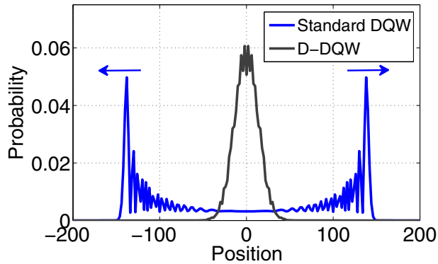
Figure 1. Probability distribution of standard DQW (with \theta = \pi/4 ) and DQW with temporal disorder after 200 steps of evolution. The initial state chosen for both the evolution, |\Psi(0)\rangle = \frac{1}{\sqrt{2}}(|\uparrow\rangle + |\downarrow\rangle) \otimes |x=0\rangle . For standard DQW, symmetric spread of wavepacket in both the direction is seen whereas, for D-DQW the wavepacket is localized around the origin.
