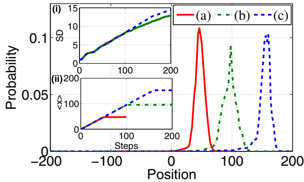
Figure 6. Probability distribution after 100 and 200 steps of DQW operation with pawl effect. For (a) [W_2]^{50}[W_1]^{50} (b) [W_2]^{100}[W_1]^{100} and (c) [W_2]^{50}[W_1]^{160} where \theta = \pi/30 for W_1 . We can see a well confined transport \propto t/2 .
