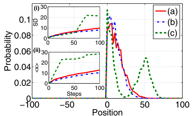
Figure 5. Probability distribution after 100 steps of DQW with pawl like effect using different order of W_1 and W_2 . For (a) W_1 with \theta = \pi/30 and W_2 are randomly picked with 1/2 probability for each step. For (b) W_1 with \theta = \pi/6 and W_2 are randomly picked with 1/2 probability for each step. For (c) W_1 with \theta = \pi/30 and W_2 are applied in order (W_2)^{25}(W_1)^{25}(W_2)^{25}(W_1)^{25} . In inset, SD and \langle x \rangle shows that the ordered combination of operations gives a better transport.
