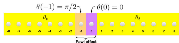
Figure 2. Schematic representation of the configuration of the evolution operation with fixed coin operations at marked positions to produce pawl like effect in DQW.
