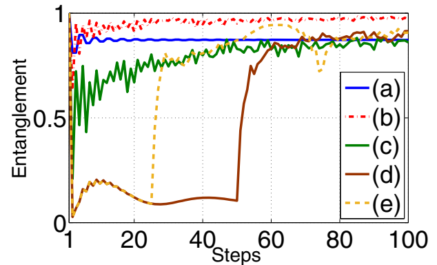
Figure 7. Entanglement with increase in number of steps for different combination of DQW with and without pawl effect. (a) and (b) are for standard DQW and D-DQW without pawl effect. (c) D-DQW with like pawl effect (d) DQW with pawl like effect using operations W_2^{50} W_1^{50} where \theta for W_1 is \pi/30 . (e) DQW with pawl like effect using operations W_2^{25} W_1^{25} W_2^{25} W_1^{25} . For all the configuration we can note that the entanglement entropy after some time reaches a values closer to 1.
