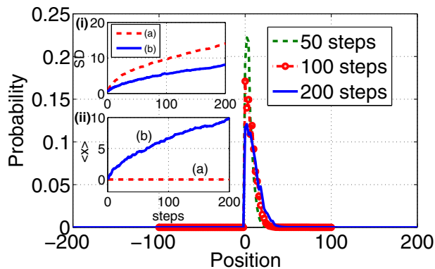
Figure 4. Probability distribution of D-DQW with pawl like effect after different number of steps. In the insets (i) and (ii) we show the standard deviation and \langle x \rangle as function of steps for D-DQW without pawl like effect in (a) and with pawl like effect in (b). We can see the increase in \langle x \rangle with pawl like effect along with a smaller standard deviation. \langle x \rangle = 0 in absence of Pawl effect.
