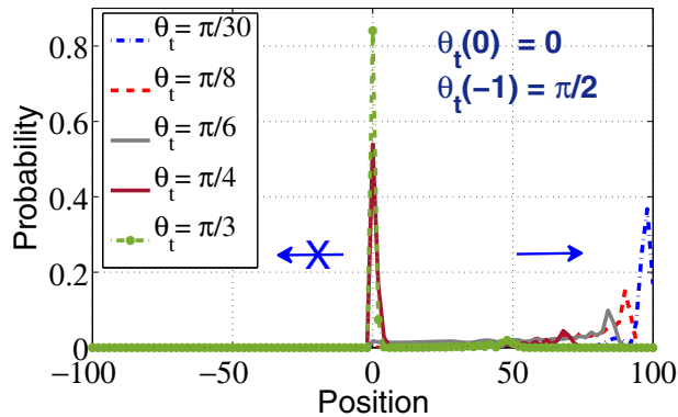
Figure 3. Probability distribution of standard DQW with \theta after 100 steps of evolution. The initial state chosen for both the evolution, |\Psi(0)\rangle = \frac{1}{\sqrt{2}}(|\uparrow\rangle + |\downarrow\rangle) \otimes |x=0\rangle . Because of the pawl like effect the wavepacket is directed towards the positive x direction for smaller value of \theta and locked around the initial position for larger value of \theta .
